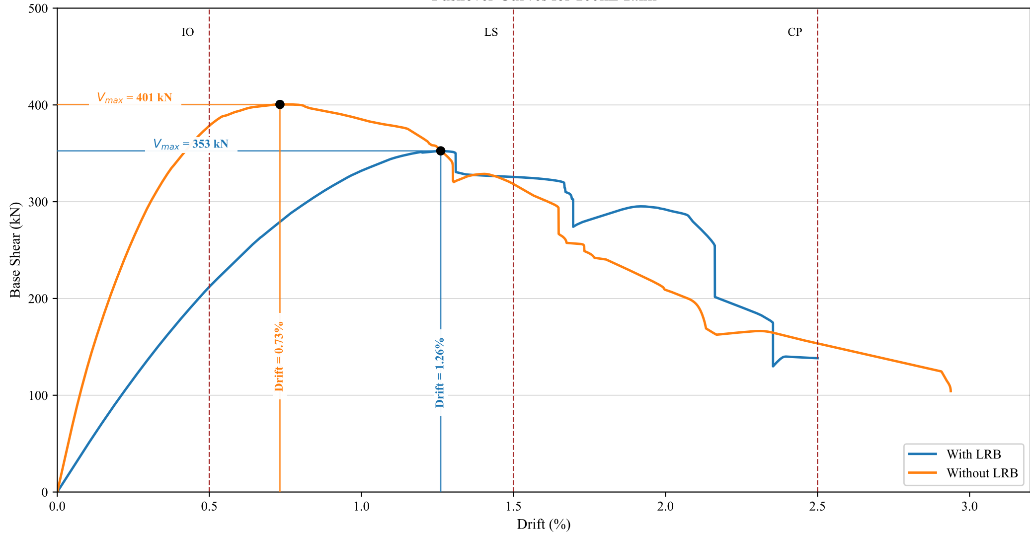
Pushover Curves for 100kL Tank
